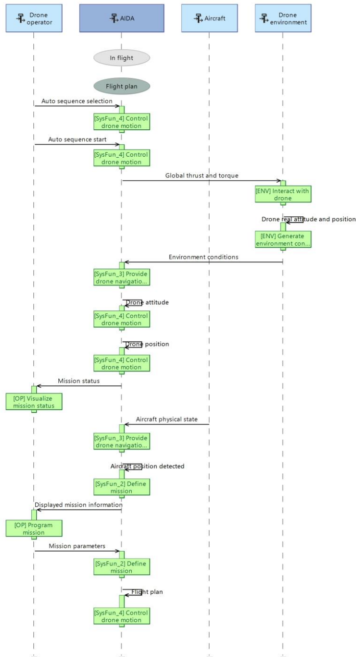
Figure 20 : "Automatic aircraft detection" sequence diagram
