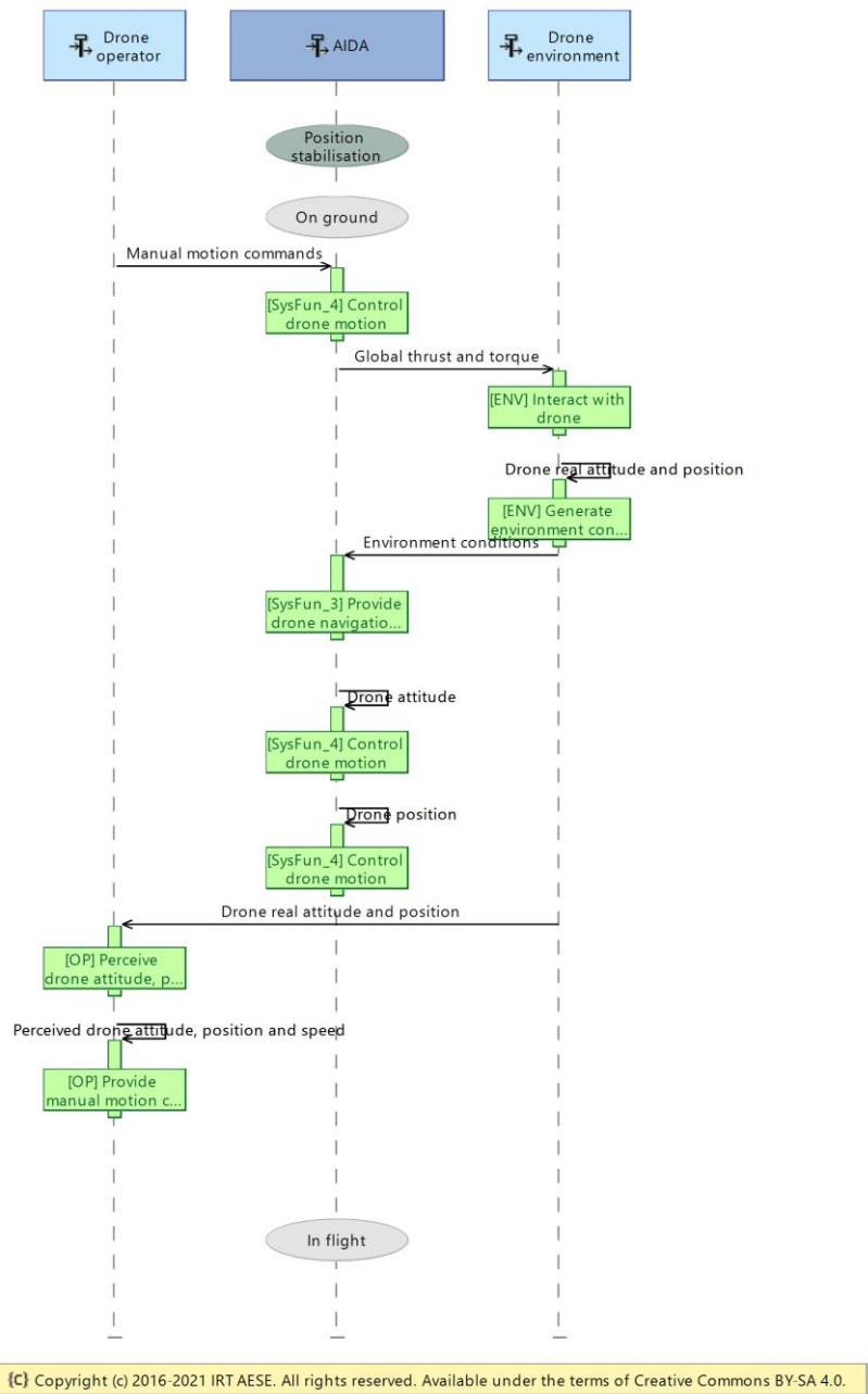
Figure 13 : "Manually control drone take off" sequence diagram
