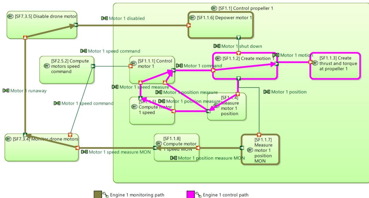
Figure 45 : SF1.X breakdown and engine control loops
