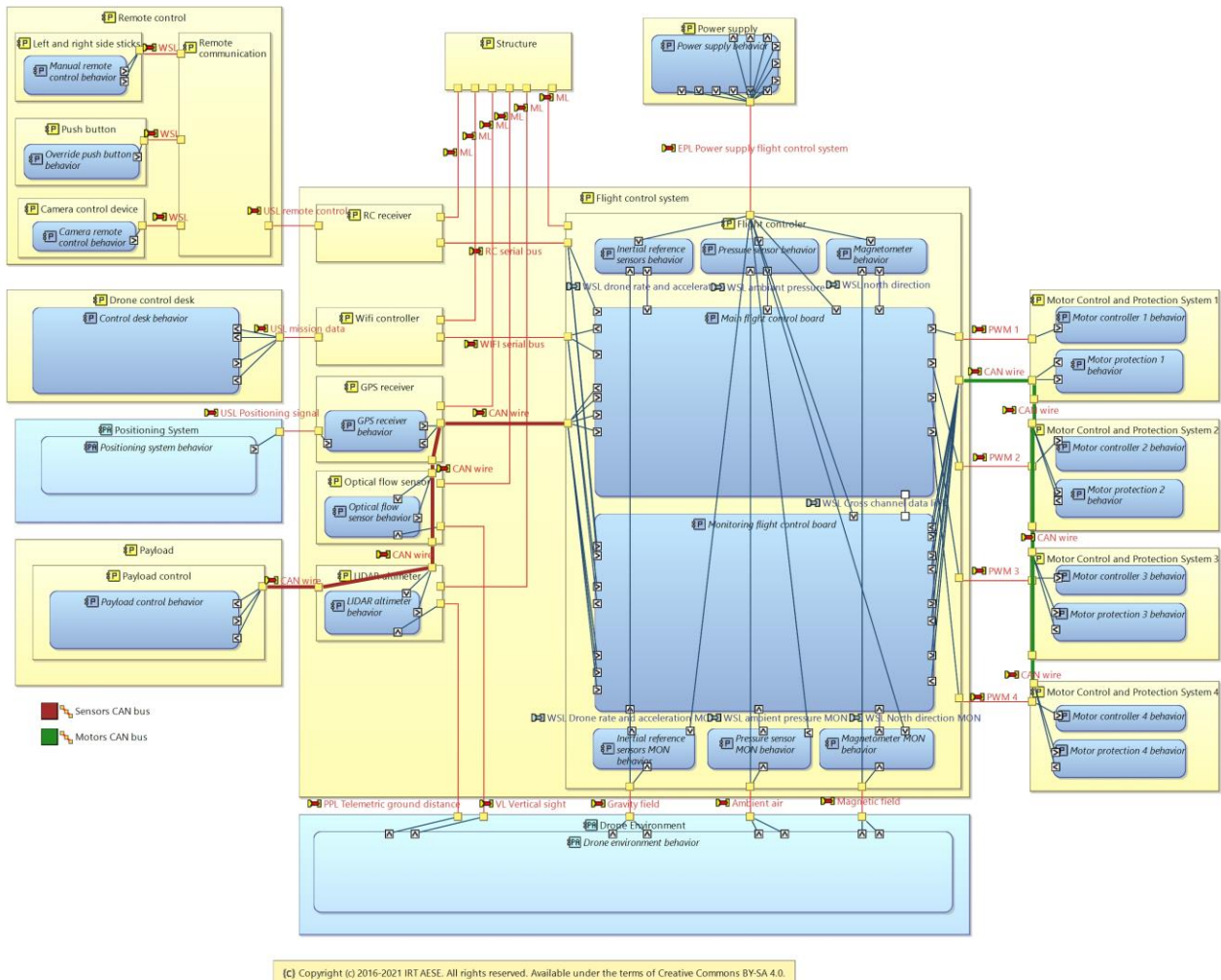
Figure 57 : Flight control system behavior components deployment
