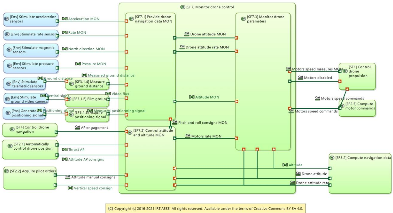
Figure 53 : SF7 breakdown
