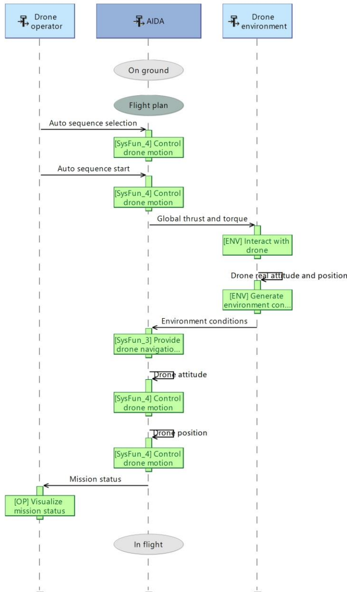
Figure 19 : "Automatic take-off" sequence diagram
