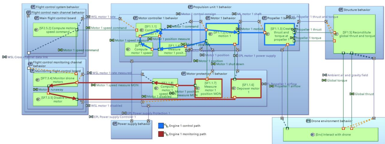
Figure 46 : Propulsion unit functional allocation
