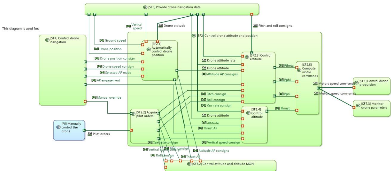
Figure 52 : SF2 breakdown
