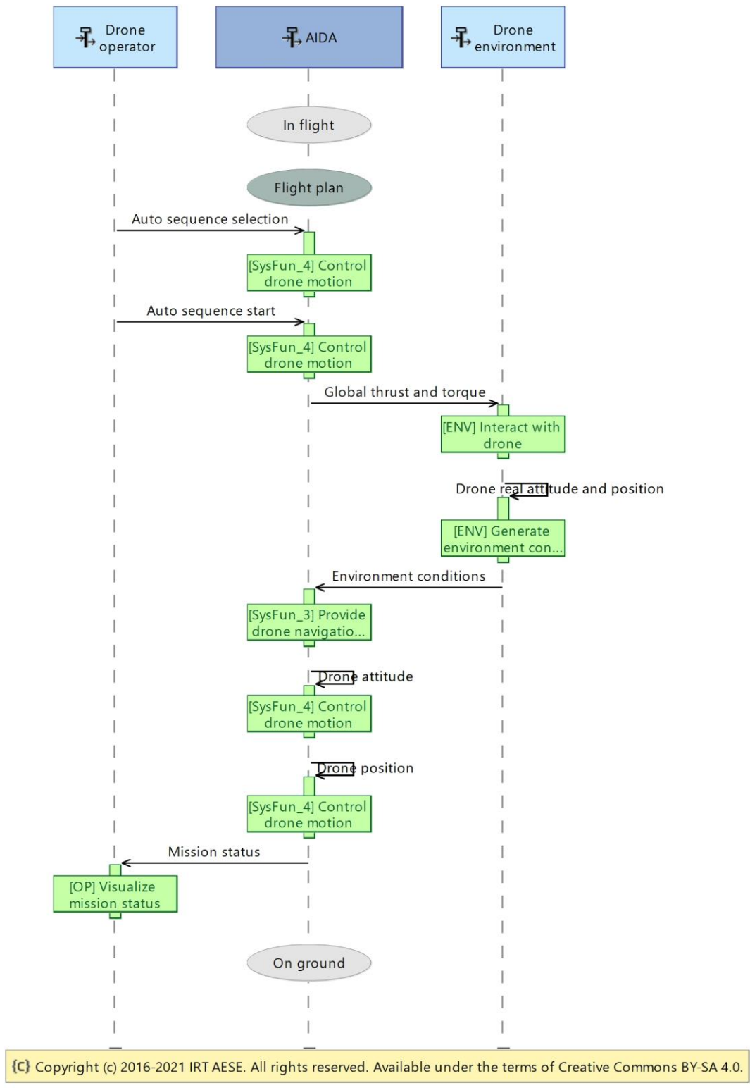
Figure 23 : "Automatic landing" sequence diagram
