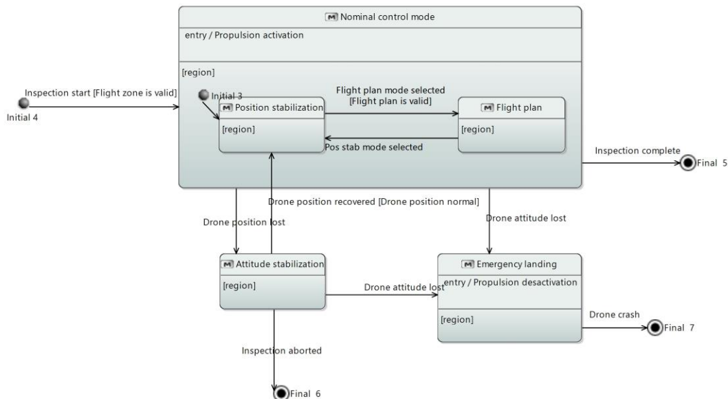
Figure 43 : control modes diagram
