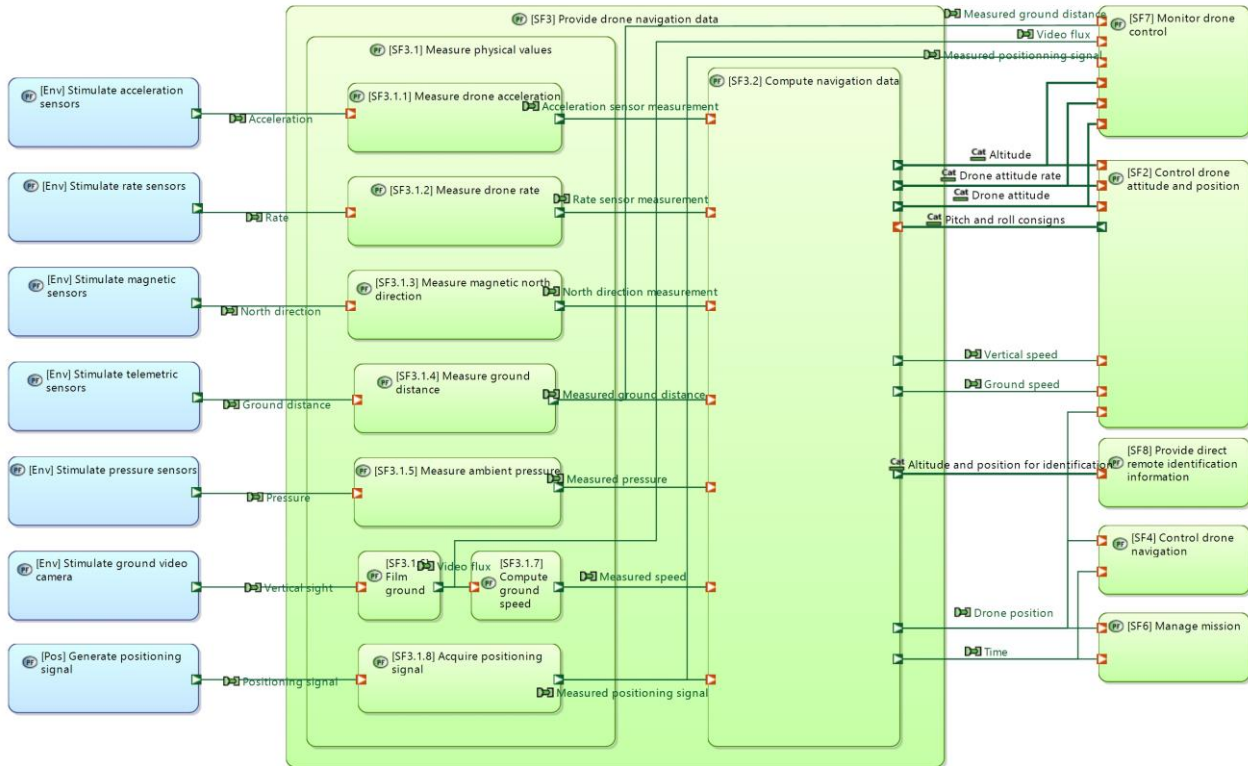
Figure 50 : SF3 breakdown
